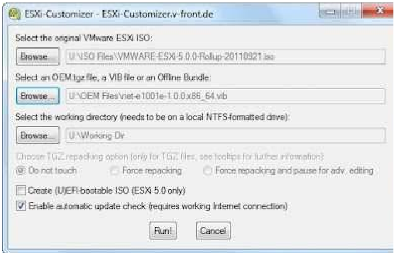
ESXi-Customizer 2.7 GUI
